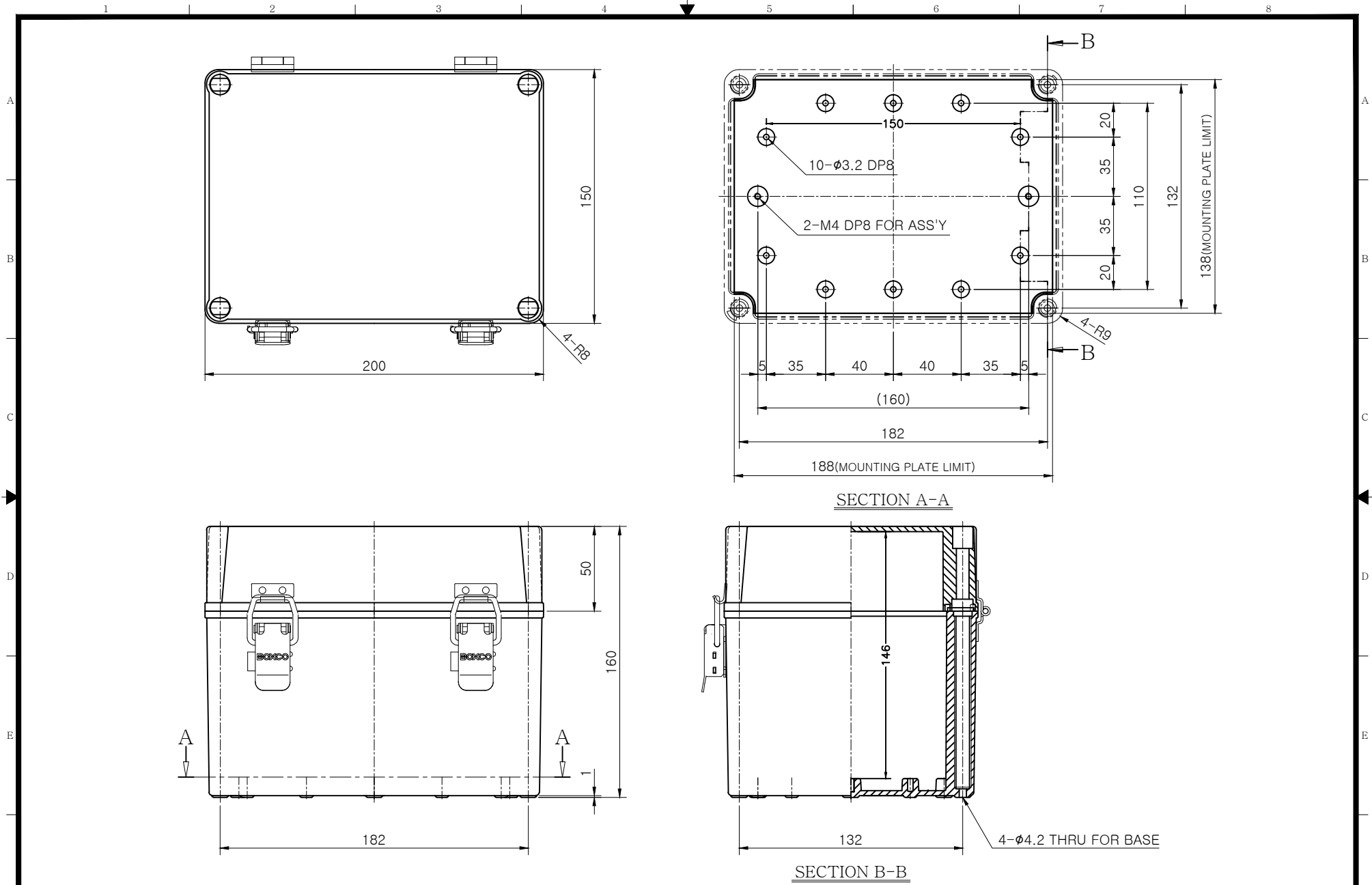
SECTION B-B
