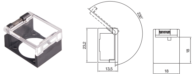
K16-S221 : Opens 230 degree
