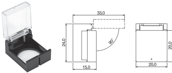
K16-S111 ① : Opens 90 degree
