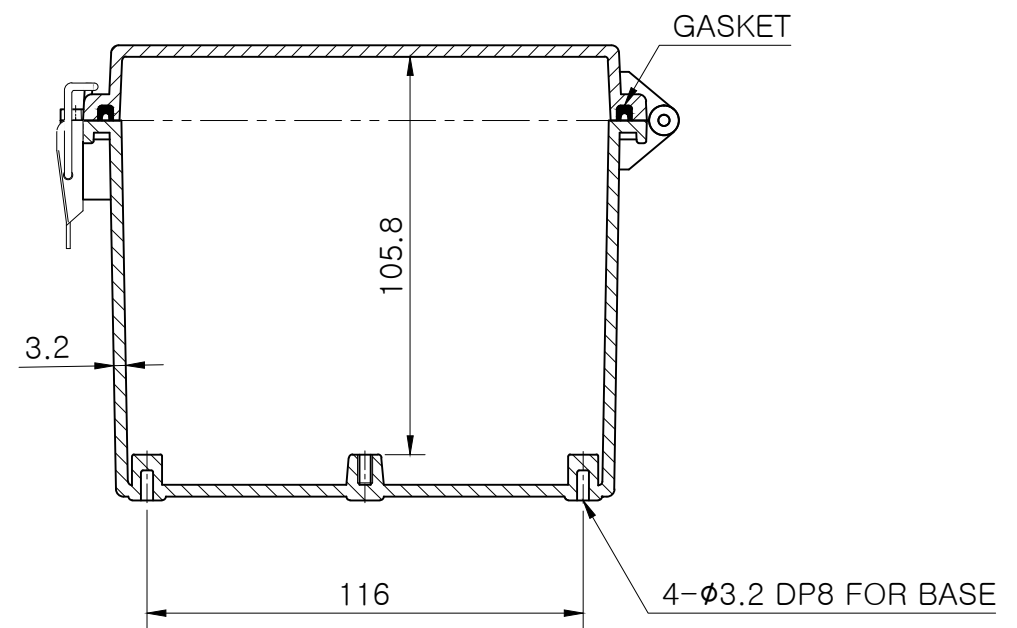
SECTION B-B
