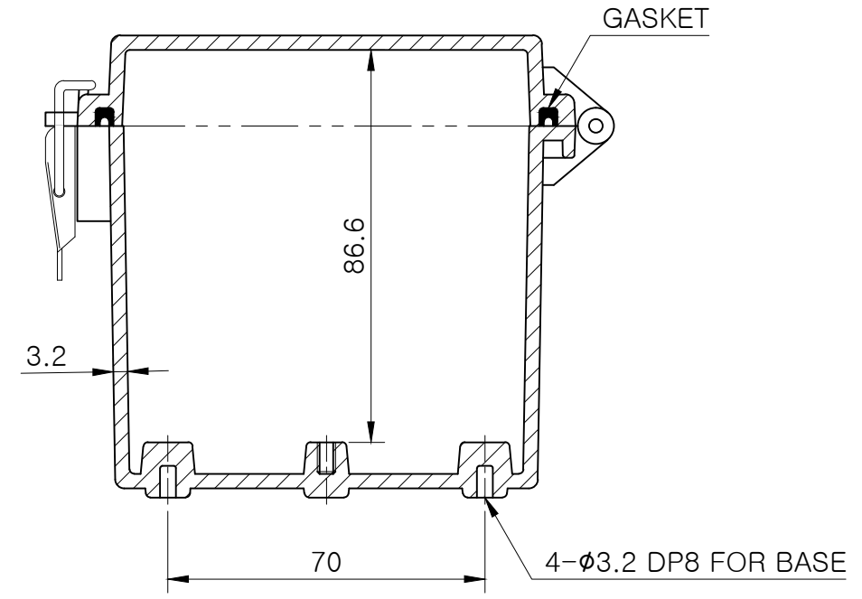
SECTION B-B
